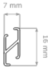
Small square end profile
