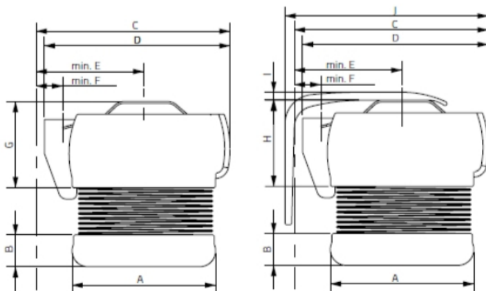
Without bracket
